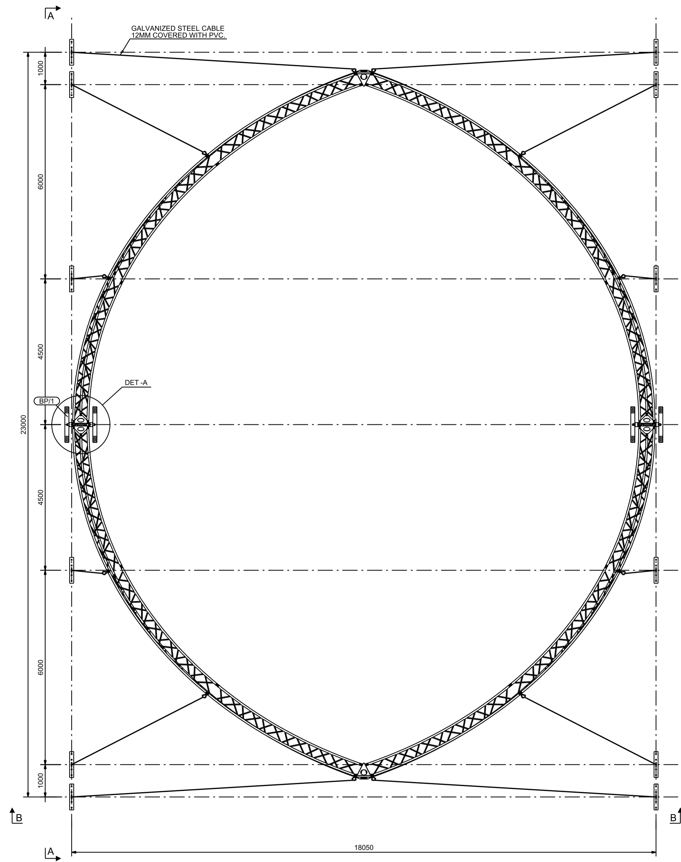
ROOF PLAN
